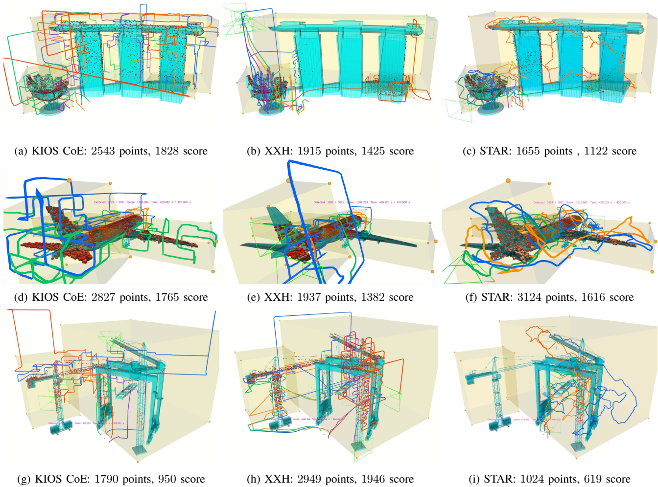
Figure 10: Illustration of the paths traveled and the points detected (red squares) for each approach for each scenario. The bounding boxes are shown in transparent yellow.
